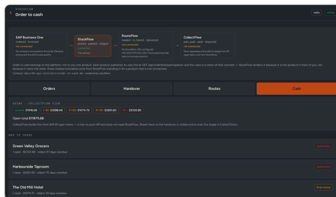
Order-to-cash across StockFlow, RouteFlow and CollectFlow
